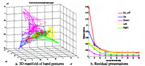
Figure 4. Distribution of dynamic hand gestures in the low-dimension.
