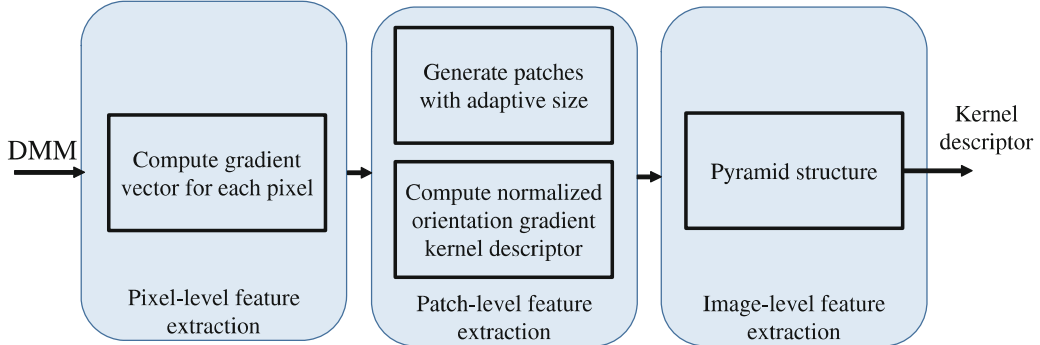
Fig. 3. Computation of kernel descriptor
